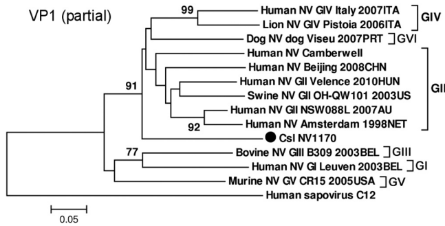
FIG. 5. Phylogenetic analysis of California sea lion norovirus (Csl NV1170) and representatives from different genogroups based on the amino acid sequence of the partial VP1 region.
