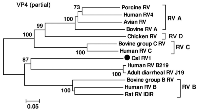
FIG. 6. Phylogenetic analysis of California sea lion rotavirus 1 (Csl RV1) and representative rotaviruses from other species based on the amino acid sequence of the partial VP4 region.
