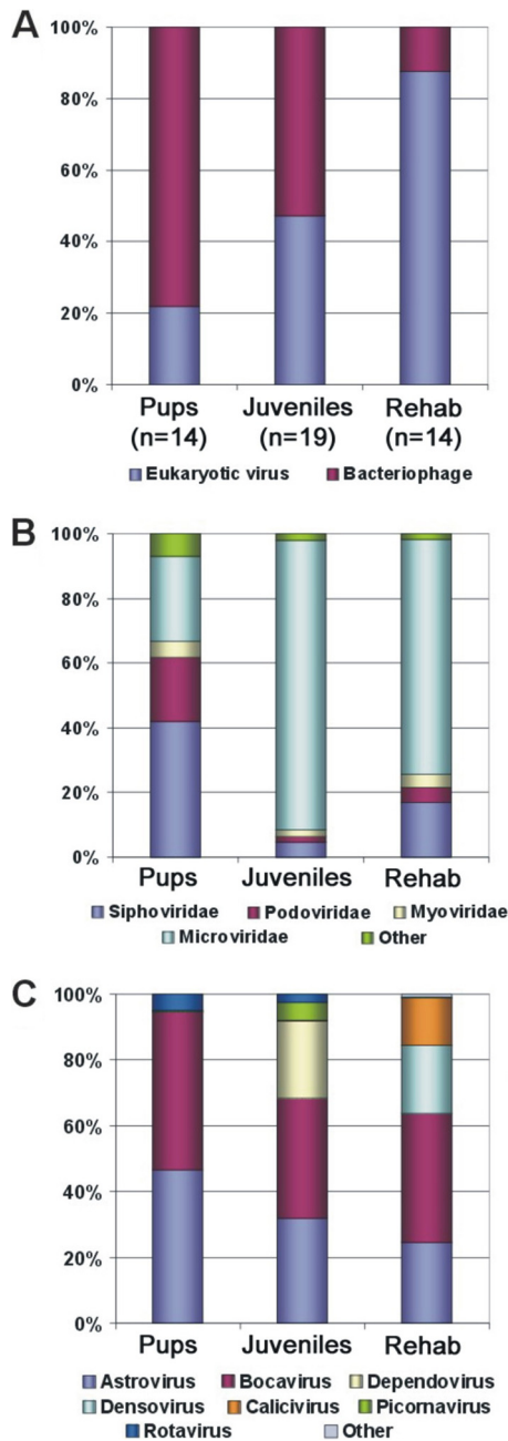
FIG. 1. Virome comparisons for three California sea lion groups based on BLASTx comparison to the GenBank nonredundant database (E value of <0.001). (A) Percentage of virus-like sequence reads with similarity to bacteriophages and eukaryotic viruses. (B) Percentage of phage-related sequences in different viral families. (C) Percentage of eukaryotic virus-related sequences in different viral groups.
