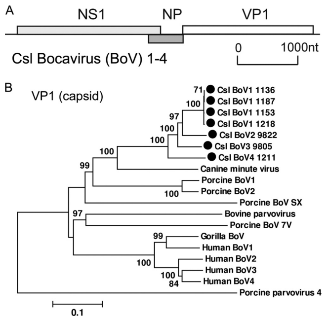
FIG. 7. (A) Genome organization of California sea lion bocaviruses (Csl BoVs). (B) Phylogenetic analysis of Csl BoVs and representative bocaviruses based on the complete VP1 protein.
